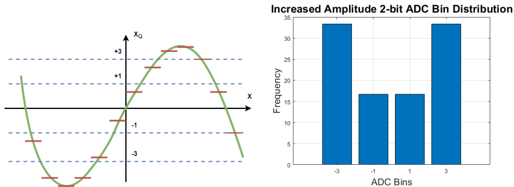
Figure 2.9: Left: Incoming signal, Right: ADC Bin Distribution
