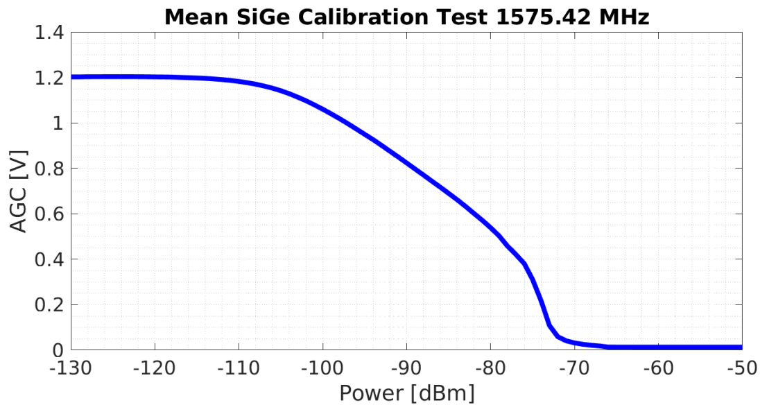
Figure 3.16: SiGe AGC power calibration curve
