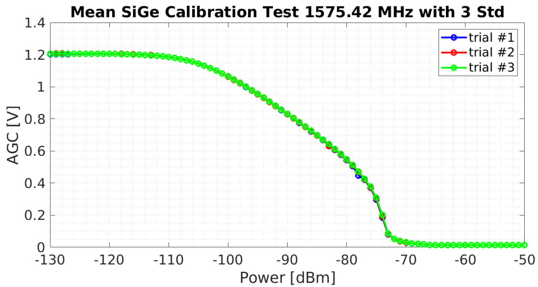
Figure 3.13: SiGe hysteresis results
